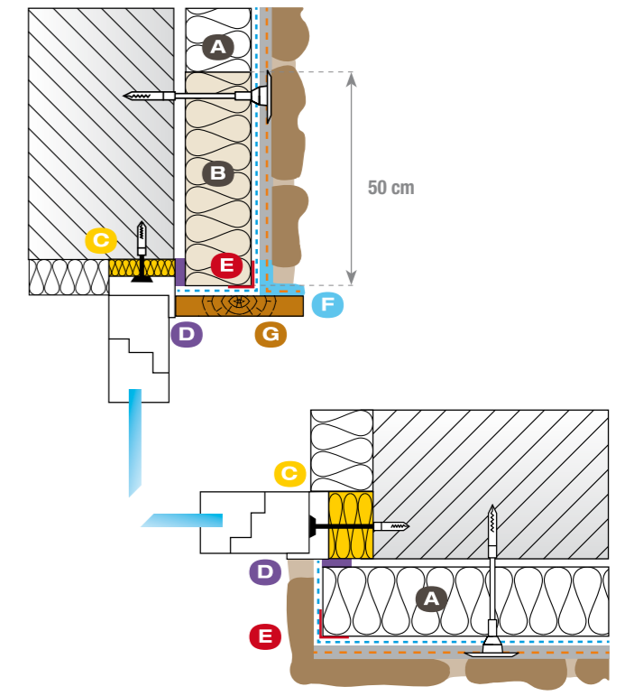
Window architrave with wooden beam
